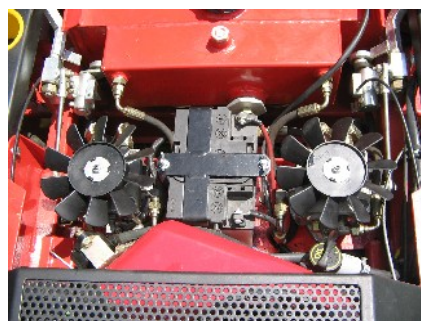
Double hydrostatic pump – one pump for each wheel moves an engine with direct transmission.
